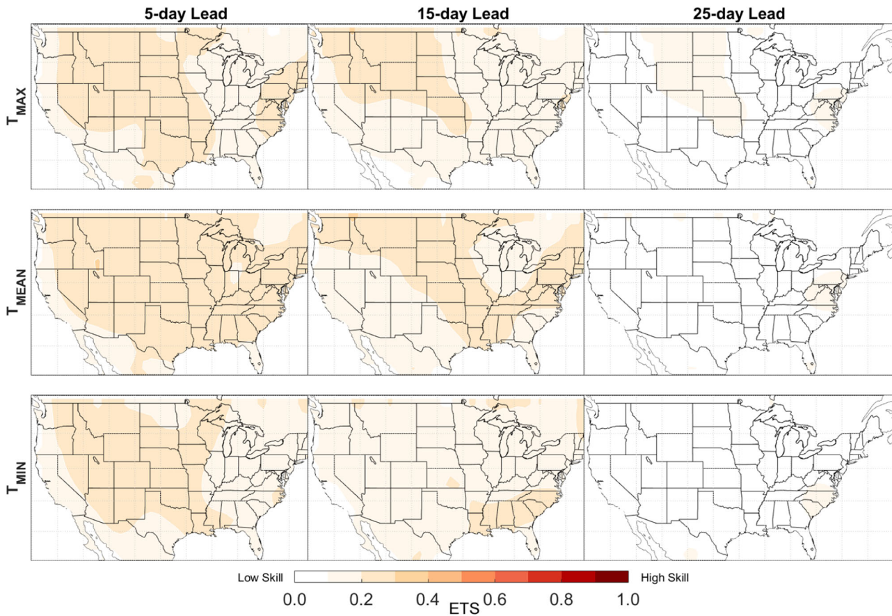
Fig. 4 Panels show areas under the equitable threat score (ETS) for heat wave forecasts validated with observations. ETS is shown of T_{\max} (top), T_{\text{mean}} (middle), and T_{\min} (bottom) at 5-day (left), 15-day (middle), and 25-day (right) lead times
